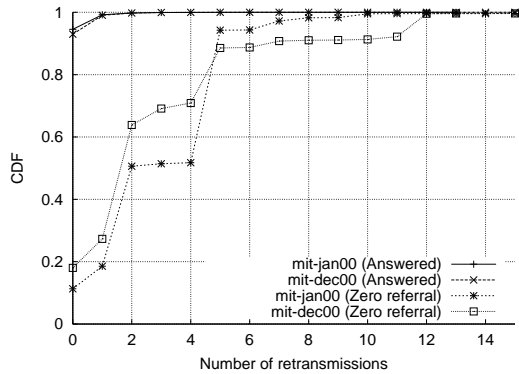
Fig. 6. Cumulative distribution of number of retransmissions for answered (top-most curves) and unanswerd lookups.
