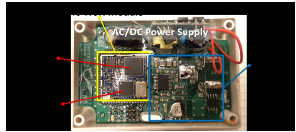
Figure 3 Interior of an ACme node
