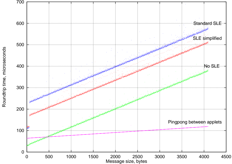
Figure 3: Round-trip latency vs. message size
