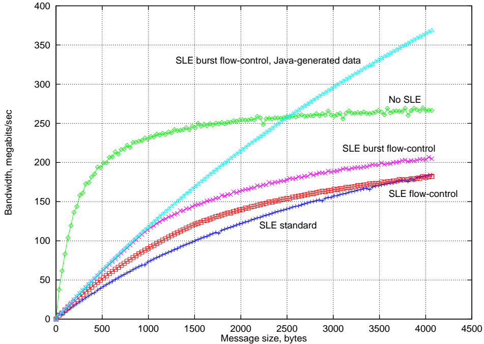
Figure 4: Bandwidth vs. message size
