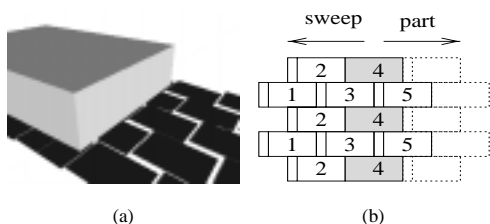
Fig. 4. The jamming problem: in (a) the part is shown unable to skip over the ridges of the encountered row of resonators. In (b) the row-strobing method is illustrated. Consecutive rows in the array are labeled from 1-8 in the direction of the part's motion (only the first 5 rows are shown). The process involves selectively turning off consecutive rows of resonators for a few oscillation cycles, in the direction opposite to the part's motion.
