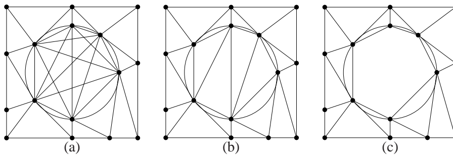
Figure 2.4: Three ways to define a Delaunay structure in the presence of cocircular vertices. (a) Include all the Delaunay simplices. (b) Choose a subset of Delaunay simplices that comprises a triangulation. (c) Exclude all crossing Delaunay edges, and fuse overlapping Delaunay triangles into Delaunay polygons.
