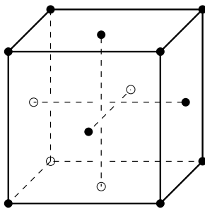
Figure 4.7: A convex PLC with no triangulation.
