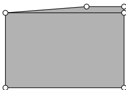
Figure 1.6: A mesh of this domain must have a new small angle.
