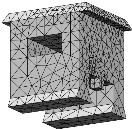
B = 1.07 , \theta_{\min} = 1.90^\circ , \theta_{\max} = 177.11^\circ , h_{\min} = 0.369 , 1397 vertices, 5596 tetrahedra.
