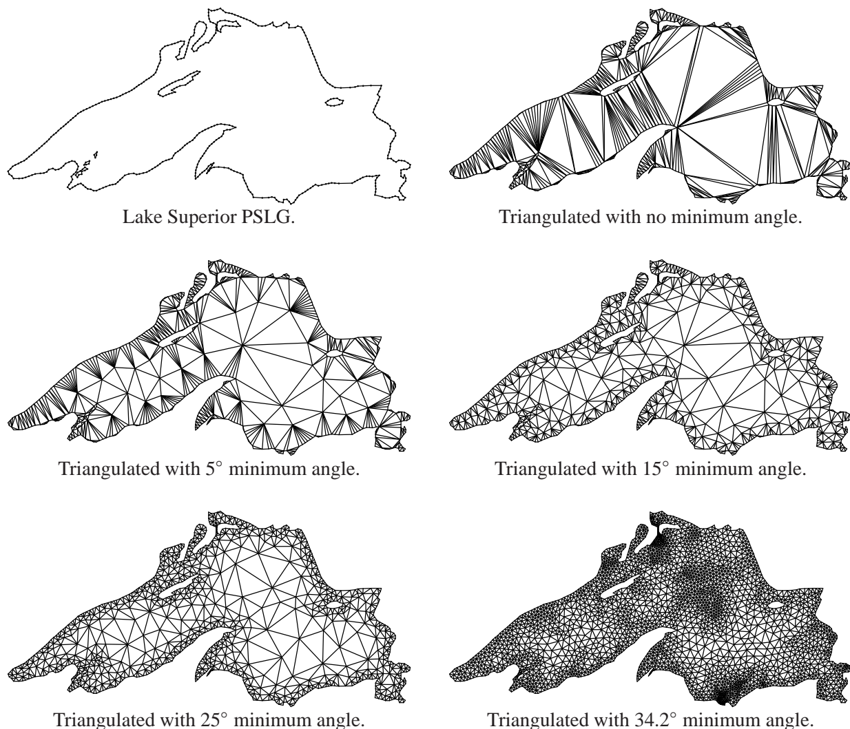
Figure 6.15: Meshes generated with Ruppert's algorithm for several different angle bounds. The algorithm does not terminate for angle bounds of 34.3^\circ or higher on this PSLG.
