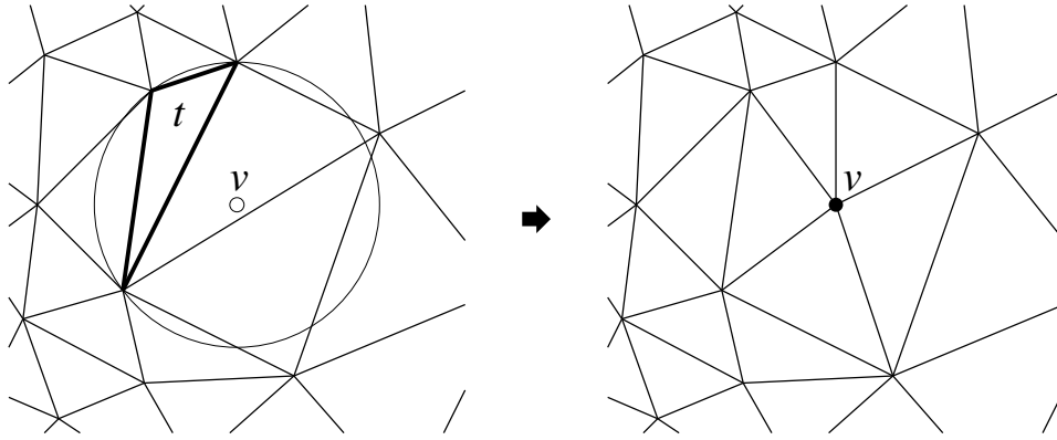
Figure 6.1: Any triangle whose circumradius-to-shortest edge ratio is larger than some bound B is split by inserting a vertex at its circumcenter. The Delaunay property is maintained, and the triangle is thus eliminated. Every new edge has length at least B times that of shortest edge of the poor triangle.
