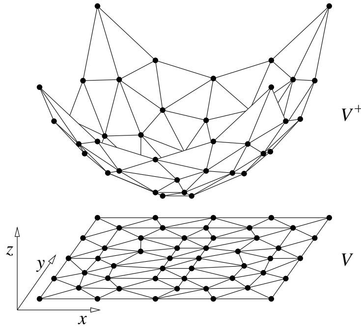
Figure 2.6: The parabolic lifting map.
