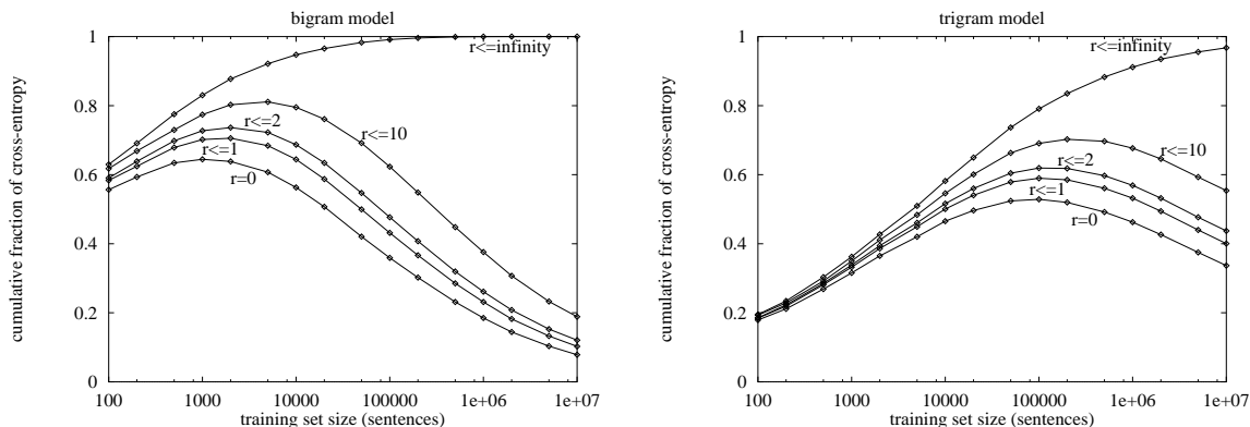
Figure 28: Cumulative fraction of cross-entropy on test set devoted to n -grams with r or fewer counts in training data for various r on WSJ/NAB corpus, jelinek-mercer-baseline smoothing, bigram and trigram models
