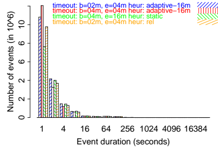
Figure 16: Event duration for various timeout heuristics .
