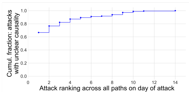
Figure 6: The ranking of attack paths with UNCLEAR causality, relative to all of the login paths that occurred on the day of an attack.
