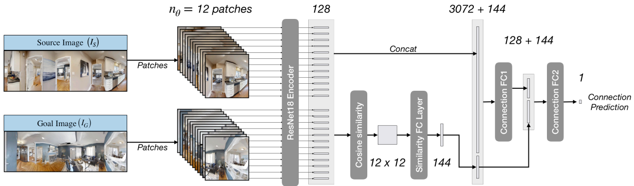
Figure 3: Connection Model. Figure showing the architecture of the Connection Model.
