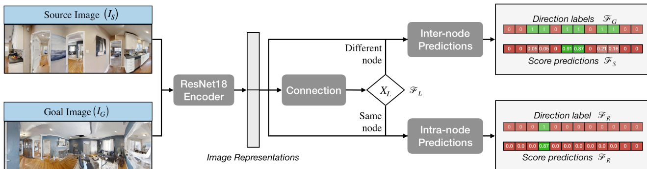
Figure 1: NTS Multi-task Learning Model. Figure showing an overview of the NTS Multi-task Learning Model. It takes a Source Image ( I_S ) and a Goal Image ( I_G ) as input and encodes them using a shared ResNet18 encoder. It first predicts whether the two images belong to the same node or not using the Connection model. If they belong to the same node, it makes Intra-Node predictions which include the direction and score (or equivalently) distance of the Goal Image relative to the Source Image. If they belong to different nodes, it makes Inter-Node Predictions which include directions of explorable areas and a semantic score corresponding to each explorable area denoting its proximity to the Goal Image.
