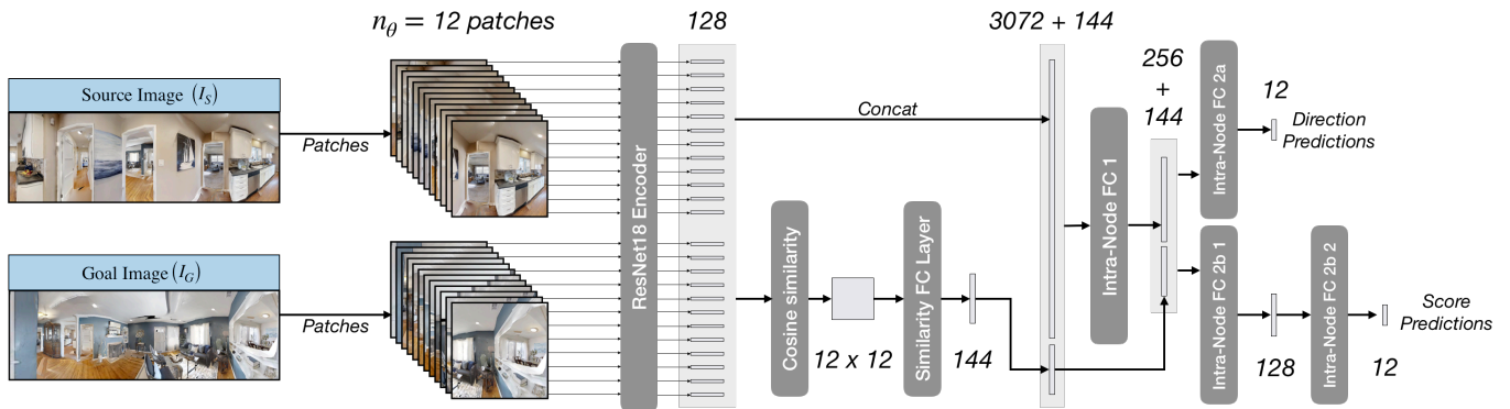
Figure 4: Intra-Node Predictions Model. Figure showing the architecture of the Intra-Node Predictions Model.
