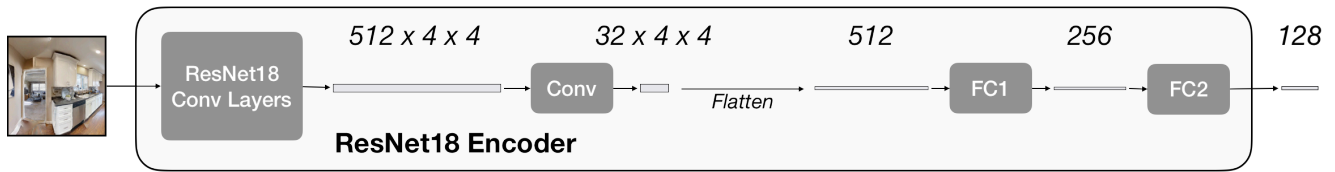
Figure 2: ResNet18 Encoder. Figure showing the architecture of the ResNet18 Encoder.
