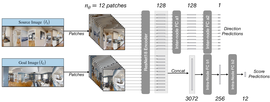
Figure 5: Inter-Node Predictions Model. Figure showing the architecture of the Inter-Node Predictions Model.
