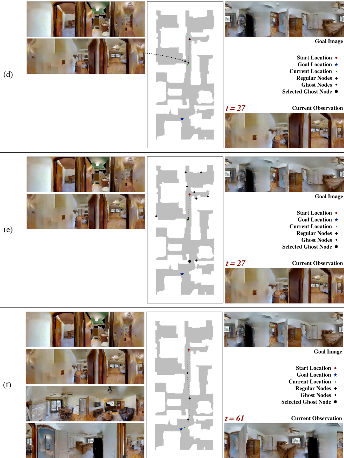
Figure 6: Example Trajectory Visualization. Figure showing a visualization of an example trajectory using the NTS model. (a) Starting and goal locations at the beginning of an episode, t = 0 shown on the ground-truth map. Note that the map is not available to the NTS model. (b) NTS model creates the first node at t = 1 . Figure showing the ghost nodes and the selected ghost node. Note that the ghost node locations are for visualization only, they are not visible or predicted by the NTS model. The model predicts only the direction of ghost nodes. (c) The agent observation at t = 20 and trajectory till t = 20 shown on the map. (d) The NTS model creates a new node at t = 27 . (e) The ghost nodes and selected ghost nodes after creating the second node. The model correctly selects the correct ghost node closest to the goal. Note that two ghost nodes in the direction of the second node from the first node are removed. (f) The agent reaches the goal at t = 61 after creating 4 nodes as shown in the trajectory on the map.
