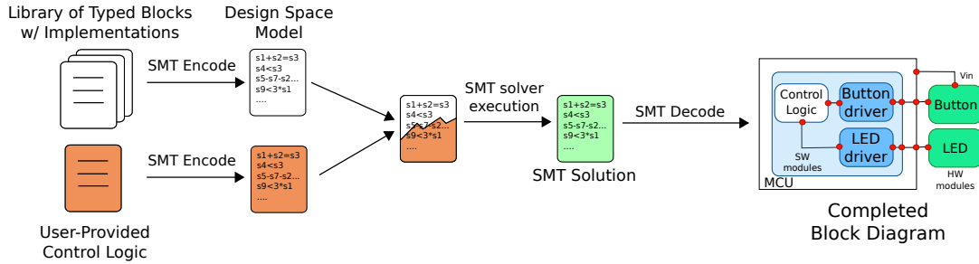
Figure 3: Design Generation at a High Level. EDG tools use existing constraint solvers to perform synthesis. The tools convert knowledge about the design space and control logic specification into constraint satisfaction problems whose solutions are block diagrams describing valid device designs. These block diagrams completely specify the design of an embedded device and can be easily converted to more useful formats.
