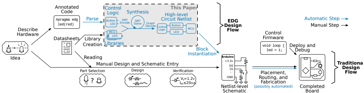
Figure 1: The Embedded Design Generation (EDG) Methodology. In contrast, with traditional embedded development methods, which rely on significant user skill, EDG only requires a high-level specification to generate an electrically correct circuit that satisfies user requirements. While EDG is a larger methodology, this paper focuses on the synthesis of high-level block diagrams from user specifications. In particular our prototype only implements those portions of the system that directly interact with the synthesis step. We both manually generate the specification needed, instead of extracting it from existing code, and manually create a circuit netlist from the output block diagram.
