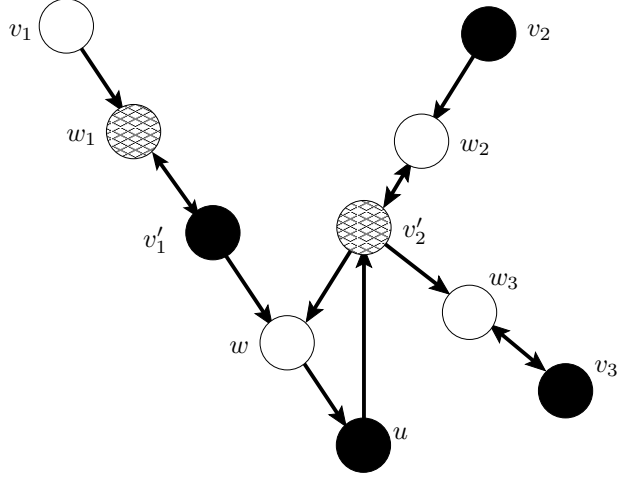
Figure 11: The new addition game and its legal 3-coloring.
