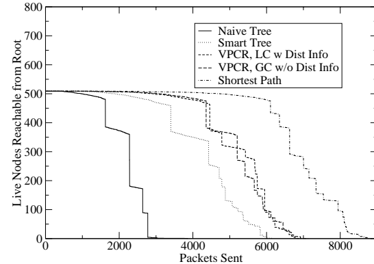
Figure 7: Network Lifetime
