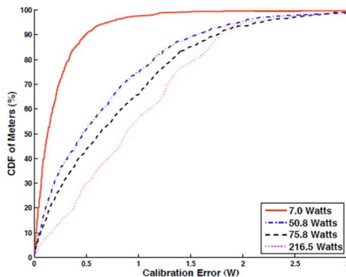
Figure 4. Error of calibrated meters at four load levels
