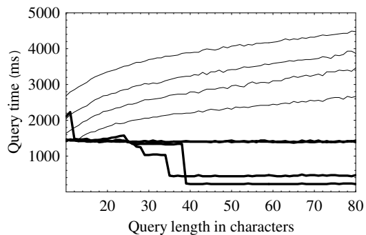
(b) chr14. From top to bottom, classical indexes (thin lines) are 7-, 8-, 9-, 10-grams, TinyLex indexes (thick lines) are 30%, 6%, 3%, 1% threshold. Query: (t)*
