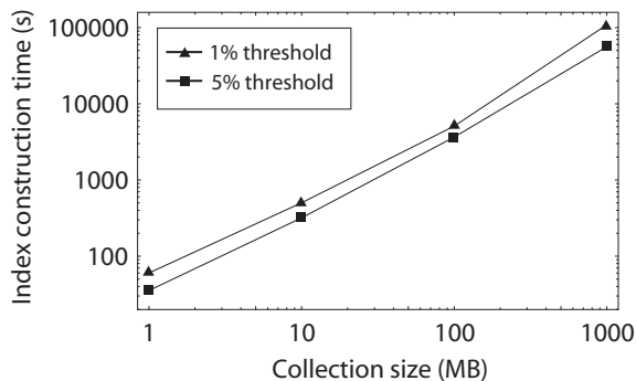
Figure 8: Scalability of TinyLex construction time at 1% and 5% threshold values over TREC collections of various sizes; scaling is roughly linear, tending up for the largest collection.
