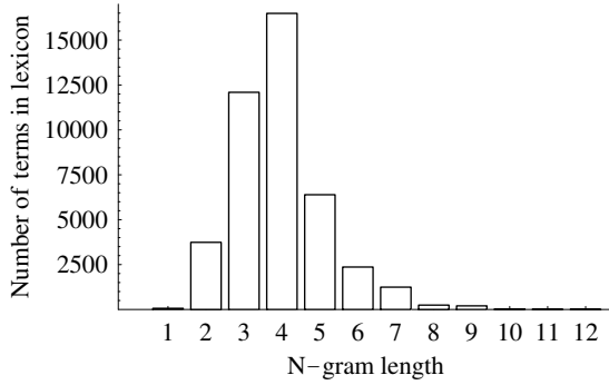
(a) Distribution of n-gram lengths on TREC-100MB collection, a typical English-language text, with 5% threshold.
