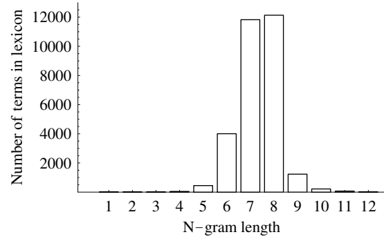
(b) Distribution of n-gram lengths on chr14 collection, a genome sequence, with 5% threshold. Omitted are 157 n-grams of length > 12.
