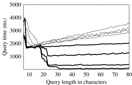
(a) TREC-100M. From top to bottom, classical indexes (thin lines) are 3-, 4-, 5-, 6-grams, TinyLex indexes (thick lines) are 50%, 7%, 2%, 0.5% threshold. Query: ( the company said)*
