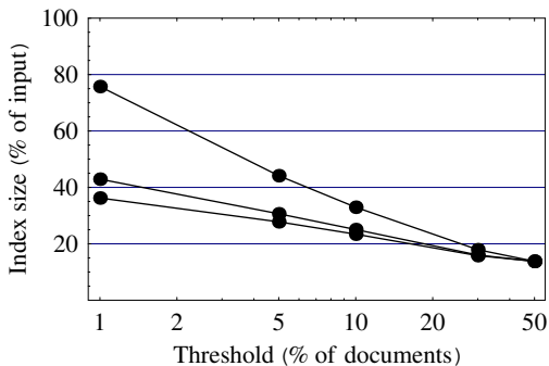
Figure 5: The impact of subset encoding on the size of the compressed posting lists for various values of the threshold parameter. From top to bottom the curves show the index size with no subset encoding, with rarest-substring subset encoding, and with full subset encoding. Data is the TREC 10MB collection. Whether or not subset compression is used, all posting lists are compressed by interpolative coding.
