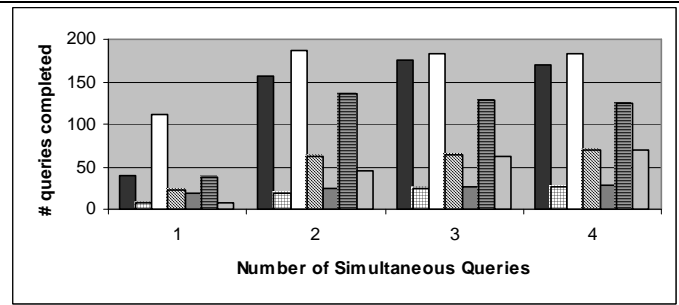
Figure 16: #queries completed within 20M tuples insertion, 75% reduction
