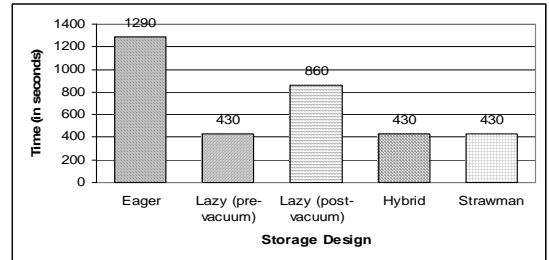
Figure 9: Time to insert 20 million tuples
