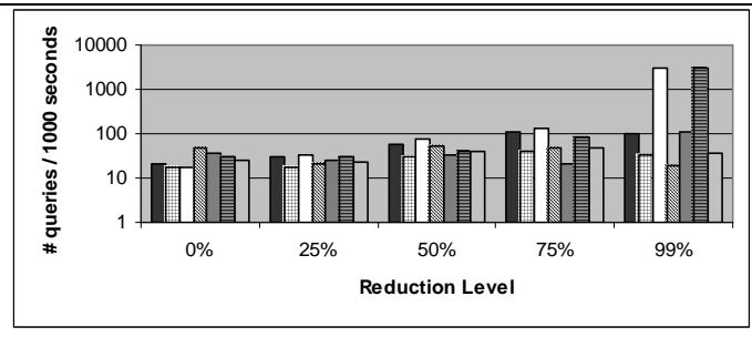
Figure 18: Queries completed/1000 sec, 4 simultaneous queries
