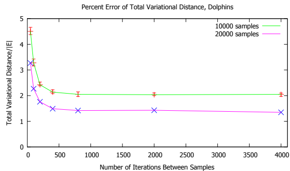
Figure 9: The total variational distance as a percentage of the sum of \mu_e . This was repeated for 10 runs with 10,000 samples each and 1 run with 20,000 samples. The error bars represent the maximum and minimum error over the 10 runs. The line is the median values.
