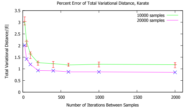
Figure 7: The total variational distance as a percentage of the sum of \mu_e . This was repeated for 10 runs with 10,000 samples each and 1 run with 20,000 samples. The error bars represent the maximum and minimum error over the 10 runs. The line is the median values.
