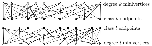
Figure 3: The JDM configuration model. This shows just two degree neighborhoods of the JDM configuration model. Each vertex of degree k is split into k minivertices which are represented by the circles. These then form a complete bipartite component when they are connected with the class k endpoints, the squares. Each degree neighborhood is completely disconnected from all others.
