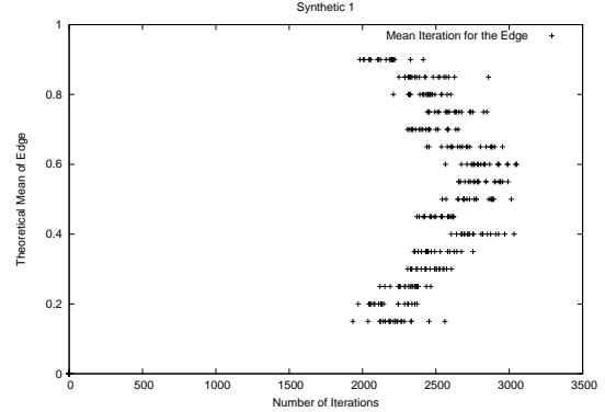
Figure 13: The time for an edge’s estimated autocorrelation function to pass under the threshold of 0.001 versus \mu_e for that edge. This synthetic dataset has a larger range of \mu_e values than the real datasets and a significant number of edges for each value.
