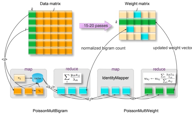
Legend: 1. Variables: x for feature counts, y for target counts, z for expected target counts, w for model weights; 2. Indices: i for feature, j for feature, k for target; 3. \langle \text{key} \rangle : distributing by a single key; 4. \langle \text{key1}, \text{key2} \rangle : distributing by a composite key.
