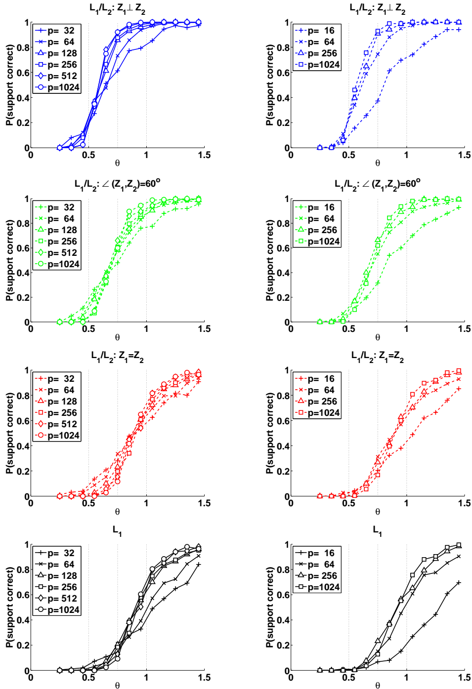
Fig 2. Plots of support union recovery probability, \mathbb{P}[\hat{S} = S] , versus the control parameter \theta = n/[2s \log(p - s)] for two different types of sparsity: linear sparsity in the left column ( s = p/8 ) and logarithmic sparsity in the right column ( s = 2 \log_2(p) ). The first three rows are based on using the multivariate group Lasso to estimate the support for the three cases of identical regression, intermediate angles and orthonormal regressions. The fourth row presents results for the Lasso in the case of identical regressions.
