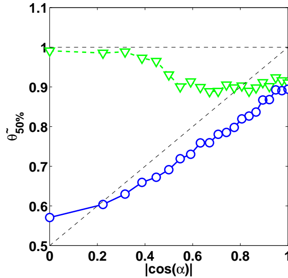
Fig 5. Plots of the Lasso sample complexity \theta = n/[2s \log(p - s)] for which the probability of support union recovery exceeds 50% empirically as a function of |\cos(\alpha)| for \ell_1 -based recovery and \ell_1/\ell_2 -based recovery, where \alpha is the angle between Z^{(1)*} and Z^{(2)*} for the family \mathcal{B}_1 . We consider the two following methods for performing row selection: Ordinary Lasso ( \ell_1 , green triangles) and multivariate group Lasso (blue circles).
