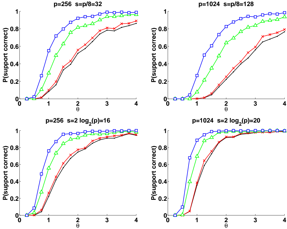
Fig 4. Plots of support recovery probability, \mathbb{P}[\widehat{S}=S] , versus the control parameter \theta = n/[2s \log(p-s)] when the covariance matrix is a Toeplitz matrix with parameter \rho = 0.5 , for the same protocol as described in Figure 3.
