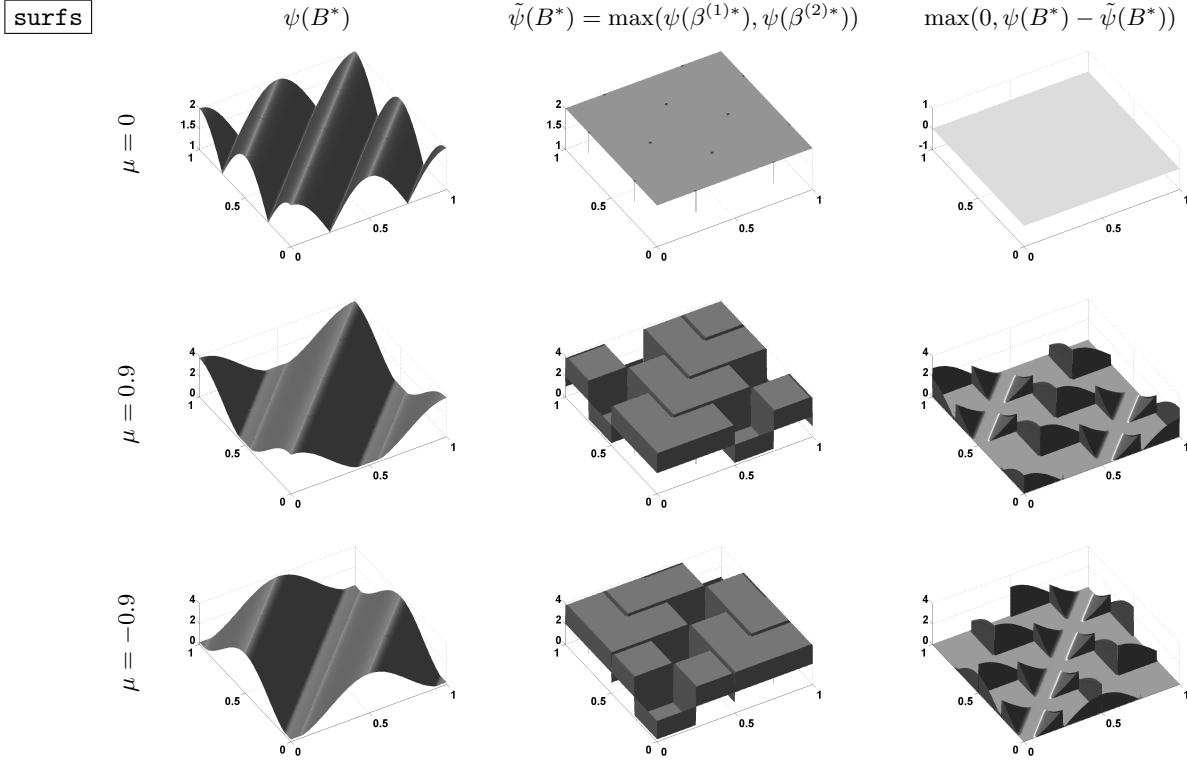
Fig 1. Comparison of sparsity-overlap functions for \ell_1/\ell_2 and the Lasso. For the pair \frac{1}{2\pi}(\vartheta_1, \vartheta_2) , we represent in each row of plots, corresponding respectively to \mu = 0 (top), 0.9 (middle) and -0.9 (bottom), from left to right, the quantities: \psi(B^*) (left), \max(\psi(\beta^{(1)*}), \psi(\beta^{(2)*})) (center) and \max(0, \psi(B^*) - \max(\psi(\beta^{(1)*}), \psi(\beta^{(2)*}))) (right). The latter indicates when the inequality \psi(B^*) \leq \max(\psi(\beta^{(1)*}), \psi(\beta^{(2)*})) does not hold and by how much it is violated.
