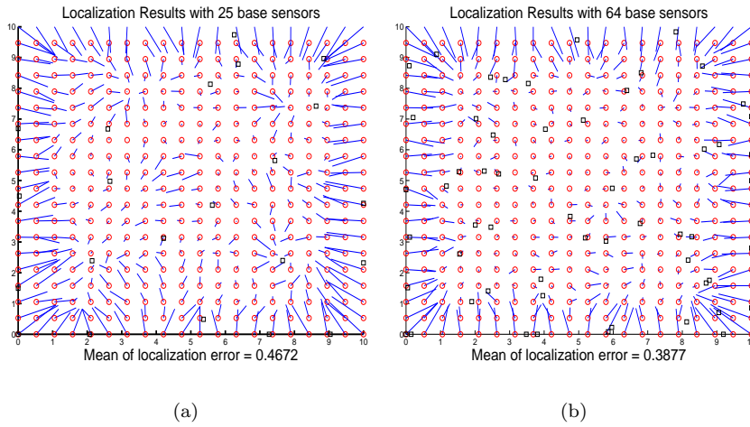
Fig. 6. Localization results for a simulated sensor network of size 10 \times 10 square units with 25 base sensors (left figure) and 64 base sensors (right figure). The base sensors are the black squares. Each blue line connects a true sensor position (in circle) and its estimate. The signal model is Gaussian. The mean localization error is 0.4672 in the left figure and 0.3877 in the right figure.
