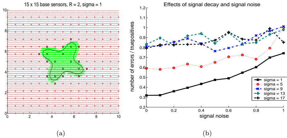
Fig. 4. (a) Illustration of a simulated sensor network with 15 \times 15 base sensors, and the recognized boundary in black (with R = 2 ) using a Gaussian kernel with \sigma = 1 . The black squares are the support vector base sensors. The test error in this figure is 0.27. (b) Plots show the effect of the sensor fading signal parameter \sigma and signal noise parameter \epsilon on coarse localization performance.
