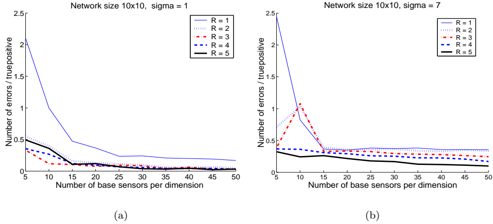
Fig. 3. Simulation results with (randomized) Gaussian models. The x -axis shows the number of sensors employed along each dimension of the network. The y -axis shows the ratio between the number of misrecognized points and the number of points inside the area to be recognized.
