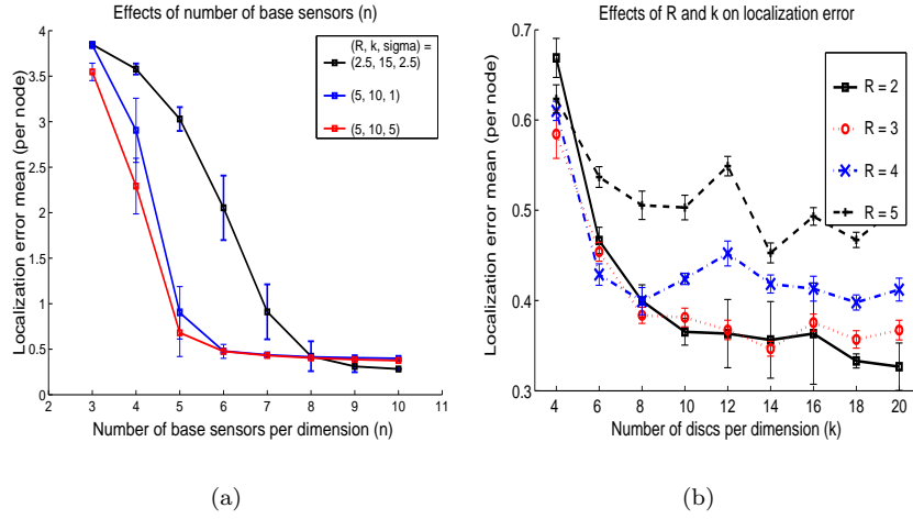
Fig. 5. Left figure shows the effect of the number of base sensors n^2 on fine-grained localization error mean and standard deviation (for all nodes). Right figure shows the effects of the size of discs (by radius R ) and the number of discs ( k^2 ) distributed uniformly on the field. The means and variances are collected after performing the simulation on 20 randomly generated sensor networks.
