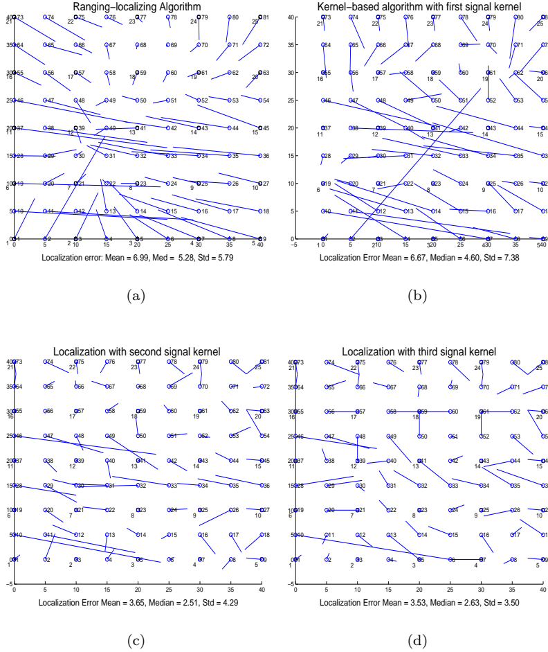
Fig. 8. Localization result for a real sensor networks covering a 40 \times 40 square-inch area. There are 25 base sensors (Berkeley notes) spaced in a 5 \times 5 grid. Each line connects a true position (in circle) and its estimate. Panel (a) shows the results given by a traditional 2-step localization algorithm, while panels (b,c,d) show the localization results obtained by our algorithm using three different kernels (the first-tier, second-tier and third-tier Gaussian kernel, respectively).
