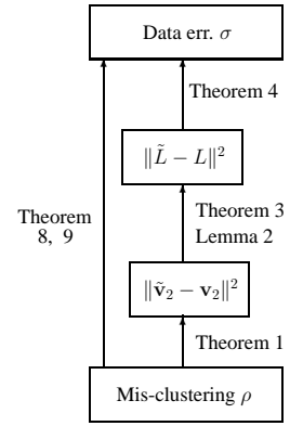
Figure 1: Data processing (top-down). Figure 2: Algorithm analysis (bottom-up).
