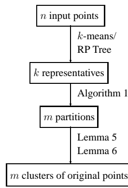
Figure 1: Data processing (top-down). Figure 2: Algorithm analysis (bottom-up).
