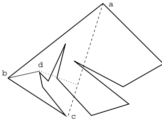
Figure 2. Finding a single diagonal.
