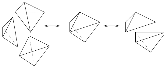
Figure 37. Two ways of tetrahedralizing five points.
