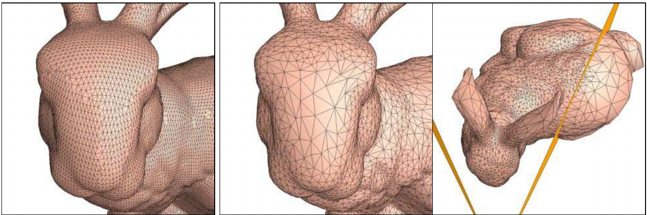
(a) Original \hat{M} (69,473 faces) (b) Front view and (c) Top view ( \tau = 0.1\% ; 10,528 faces)
