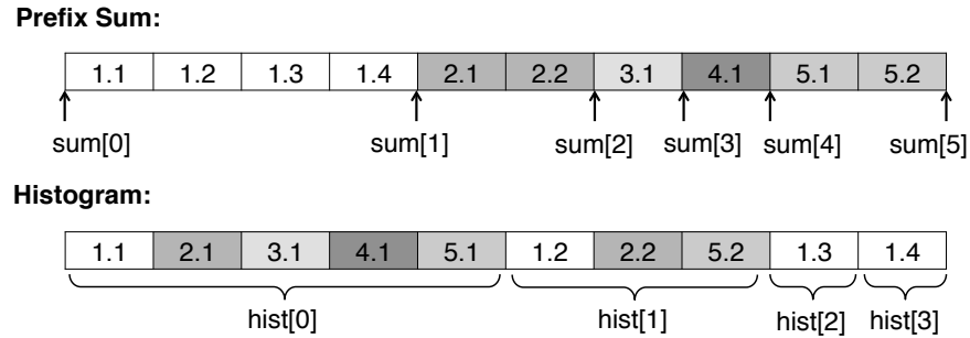
Figure 6.8: Comparing our two different approaches for calculating offsets. m.n describes the n 'th reference of the m 'th object (i.e. work-item).
