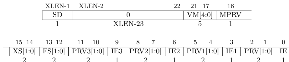
Figure 3.4: Machine-mode status register ( mstatus ).
