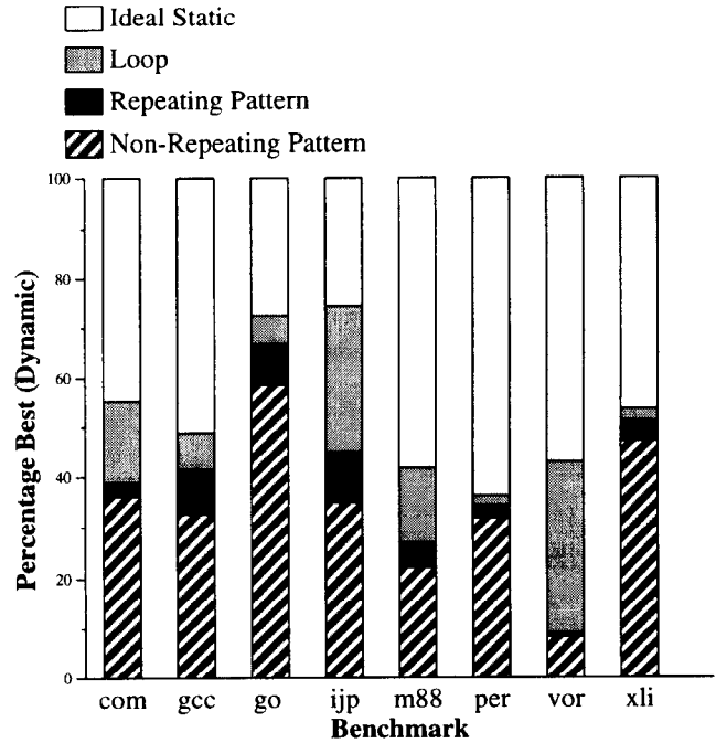
Figure 6. Fraction of branches each per-address class was dominant weighted by the dynamic execution frequencies of the branches
