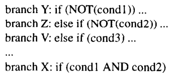
Figure 2. Example of in-path correlation
