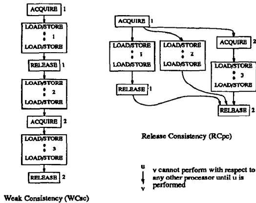
Figure 4: Possible overlap difference between WCsc and RCpc.
