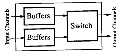
Fig. 6. Node organization. Each network node contains a set of buffers for each input channel and a switch.
