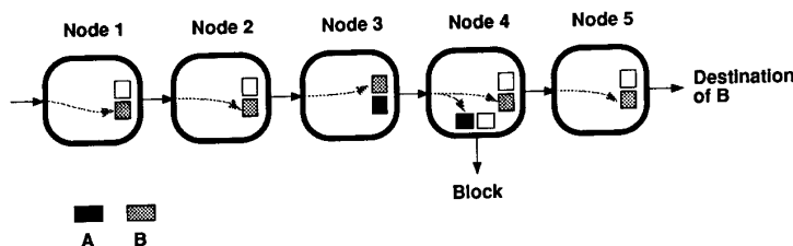
Fig. 2. Virtual channels provide additional buffers allowing packet B to pass blocked packet A.
