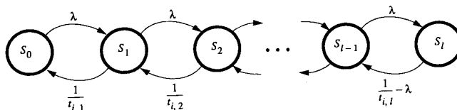
Fig. 10. Virtual channel occupancy probabilities are calculated using a Markov model. State S_j corresponds to j virtual channels being occupied.
