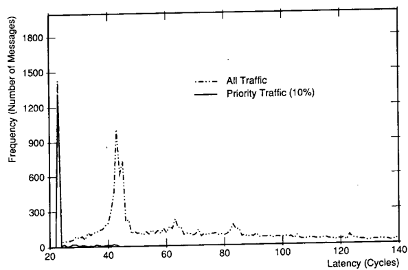
Fig. 18. Latency histogram for a 2-ary 6-fly network with random traffic at 50% capacity where 10% of the traffic is marked high-priority and scheduled by age. 80% of the high-priority traffic is delivered with the minimum latency.
