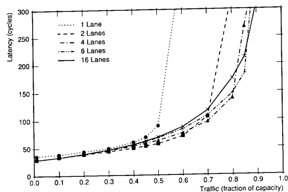
Fig. 19. Latency versus offered traffic for 16-ary 2-cube mesh networks under random traffic. As with the butterfly networks, adding lanes to a network has little effect on latency below the saturation throughput for a single lane. Adding a lane dramatically increases throughput at first with diminishing returns for 8 and 16 lanes.
