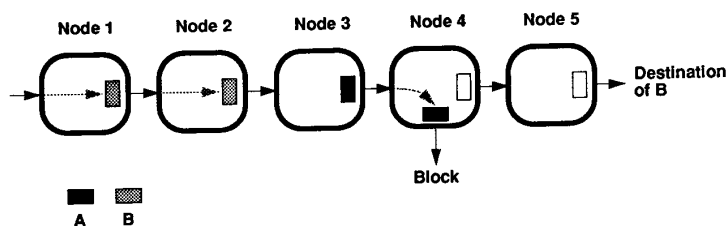
Fig. 1. Packet B is blocked behind packet A while all physical channels remain idle.
