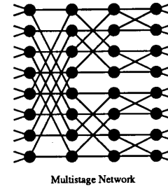
Fig. 4. A 2-ary 4-fly network.
