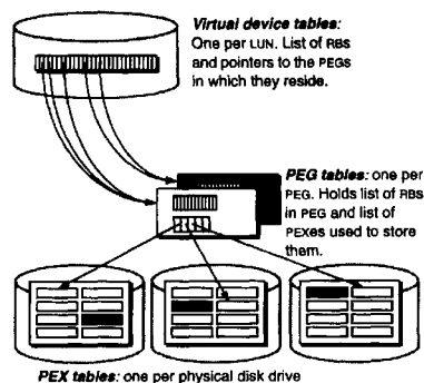
Fig. 5. Structure of the tables that map addresses in virtual volumes to PEGs, PEXEs, and physical disk addresses (simplified).
