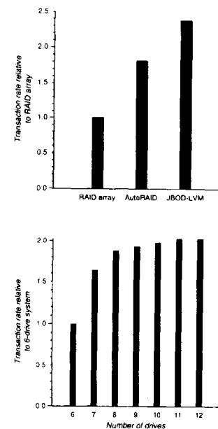
Fig. 6. OLTP macrobenchmark results; (a) comparison of HP AutoRAID and non-RAID drives with a regular RAID array. Each system used 12 drives, and the entire 6.7GB database fit in mirrored storage in HP AutoRAID; (b) performance of HP AutoRAID when different numbers of drives are used. The fraction of the 8.1GB database held in mirrored storage was: 1/3 in the 6-drive system, 2/3 in the 7-drive system, nearly all in the 8-drive system, and all in the larger systems.
