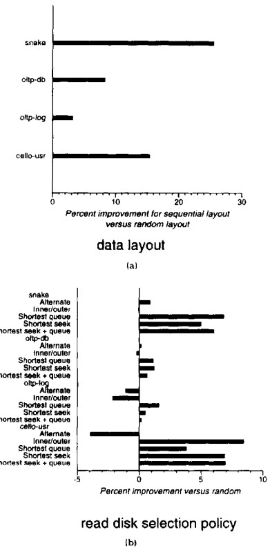
Fig. 9. Effects of (a) data layout and (b) mirrored storage class read disk selection policy on performance.
