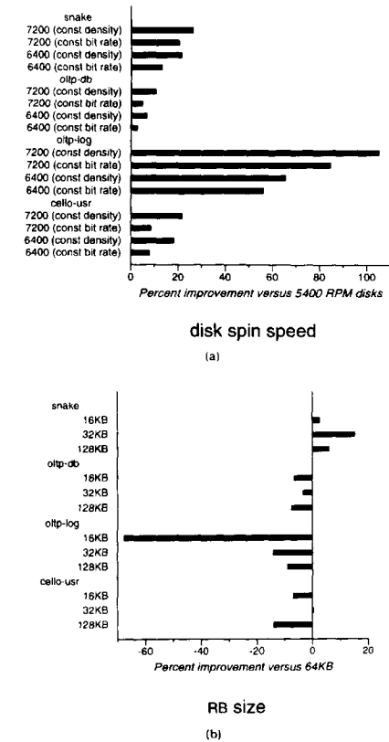
Fig. 8. Effects of (a) disk spin speed and (b) RB size on performance.
