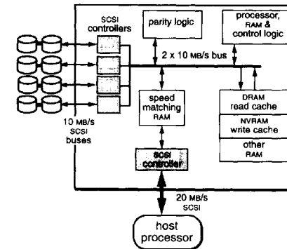
Fig. 2. Overview of HP AutoRAID hardware.
