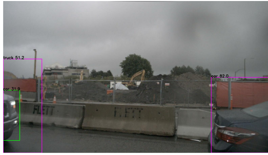
Fig. 5. Example of a model prediction error in the nuScenes autonomous vehicle dataset. This error was found via a consistency assertion between different sensor views of the same data (3D point cloud and camera data). Taken from Kang et al. [32].
