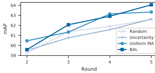
Fig. 7. Performance of active learning when using random sampling, uncertainty sampling, and model assertions. BAL is the bandit active learning algorithm that leverages model assertions. The x -axis is the round of training, and the y -axis is the mAP. As shown, BAL can achieve the 62 mAP target with 40% fewer labels compared to baselines. Taken from Kang et al. [32].
