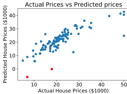
Fig. 4. Example of errors when predicting housing prices. As we can see, two of the examples are predicted as having negative housing prices, which is infeasible.
