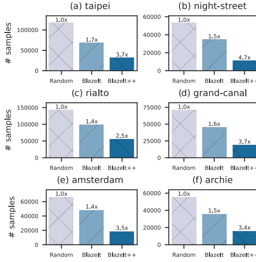
Fig. 8. Performance of BLAZEIT and BLAZEIT++ on the datasets considered by Kang et al. [25]. The y -axis is the number of samples required to achieve the error target. We show the improvement over random sampling in the numbers above the bars. As shown, our improved algorithm outperforms on all datasets.
