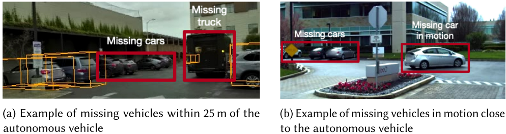
Fig. 3. Examples of errors from the publicly available Lyft Level 5 dataset. This dataset was produced by a leading labeling vendor. Taken from Kang et al. [24].
