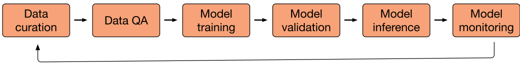
Fig. 1. Steps present in most ML deployments. Most of the literature focuses on model training, validation, and inference. Furthermore, most of the data assumes the pipeline is fixed, as opposed to ongoing. We argue for the importance of the underlooked components of the ML deployment pipeline: data curation, data quality assurance, and model monitoring.
