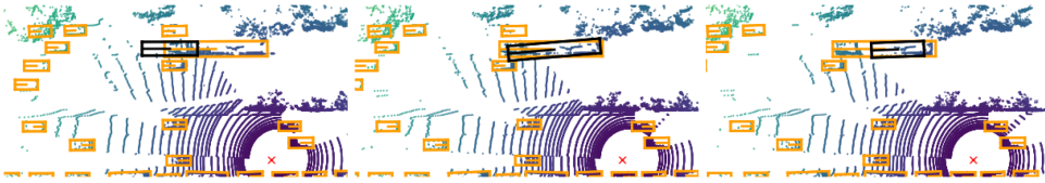
Fig. 6. Example of a model prediction error on the Lyft Level 5 dataset. Although the predicted boxes (in black) overlap with the ground truth boxes (in orange), they are inconsistent over time and can be found with FIXY as a result. Taken from Kang et al. [24].
