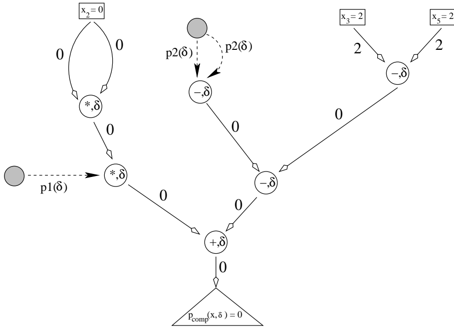
Figure 2: The three ways to produce zeros.
