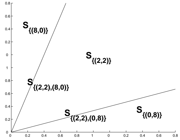
Figure 4: The intersection -N(P) \cap \mathbb{R}_+^k and the regions S_{\Lambda_j} .
