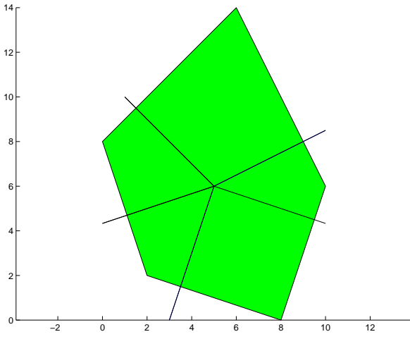
Figure 3: The Newton polytope P and its normal fan N(P) for Example 3.20.
