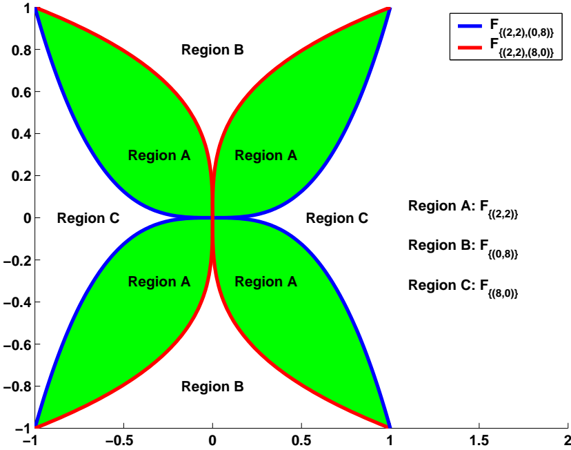
Figure 5: The regions F_{\Lambda_j} .
