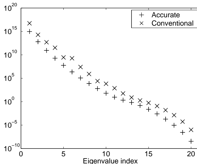
Figure 1: Eigenvalues of the 20th Schur Complement of the 40-by-40 Vandermonde matrix V_{ij} = i^{j-1} , computed both using a Conventional algorithm (x) and an Accurate algorithm (+).
