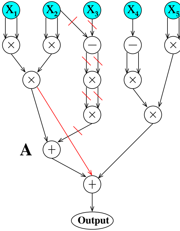
Figure 6: Pruning an algorithm for p(x) = x_1^2 x_2^2 + (x_2 - x_3)^4 + (x_3 - x_4)^2 x_5^2 .
