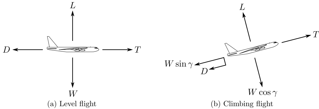
Figure 5.1: Force balances in steady flight.
