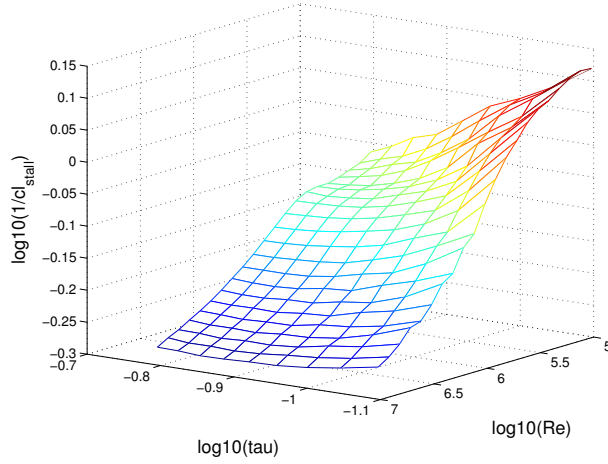
Figure 5.8: NACA-00xx series stall point data from XFOIL, plotted on a log scale. The data is not log-convex, but a single monomial plane provides a reasonable approximation. Here the z -axis is 1/C_{L,\max} . Unlike drag, high values of C_{L,\max} are actually desirable, so it is 1/C_{L,\max} that we seek a log-convex (or log-affine, in this case) model for.
