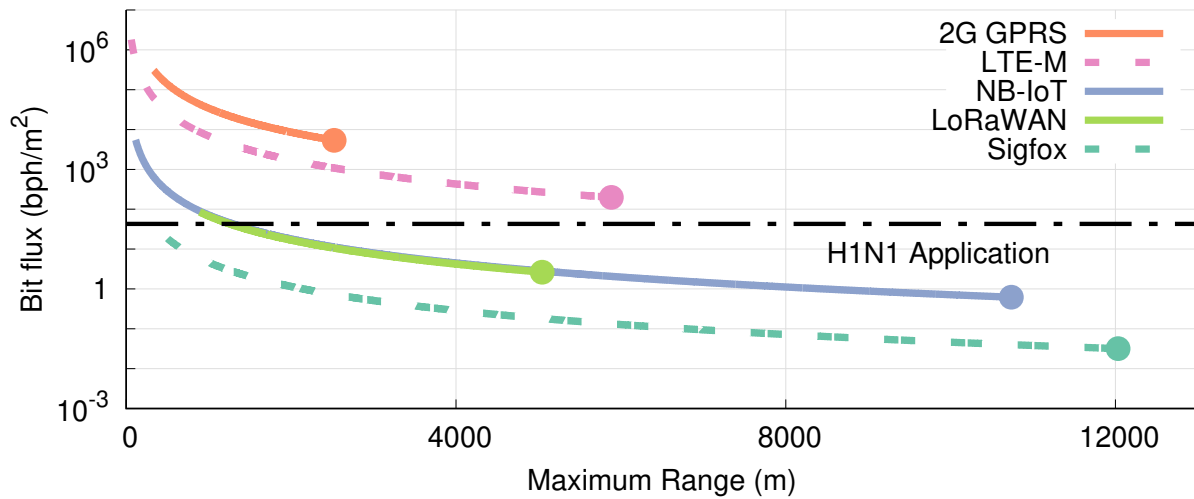
Figure 7.1: Bit flux for networks and the H1N1 application. LTE-M satisfies application needs, but only while devoting most of the network to the application. NB-IoT and LoRaWAN are capable of satisfying application needs with range reduction and the deployment of additional gateways. Sigfox is incapable of meeting the needs of the H1N1 application under any configuration.
