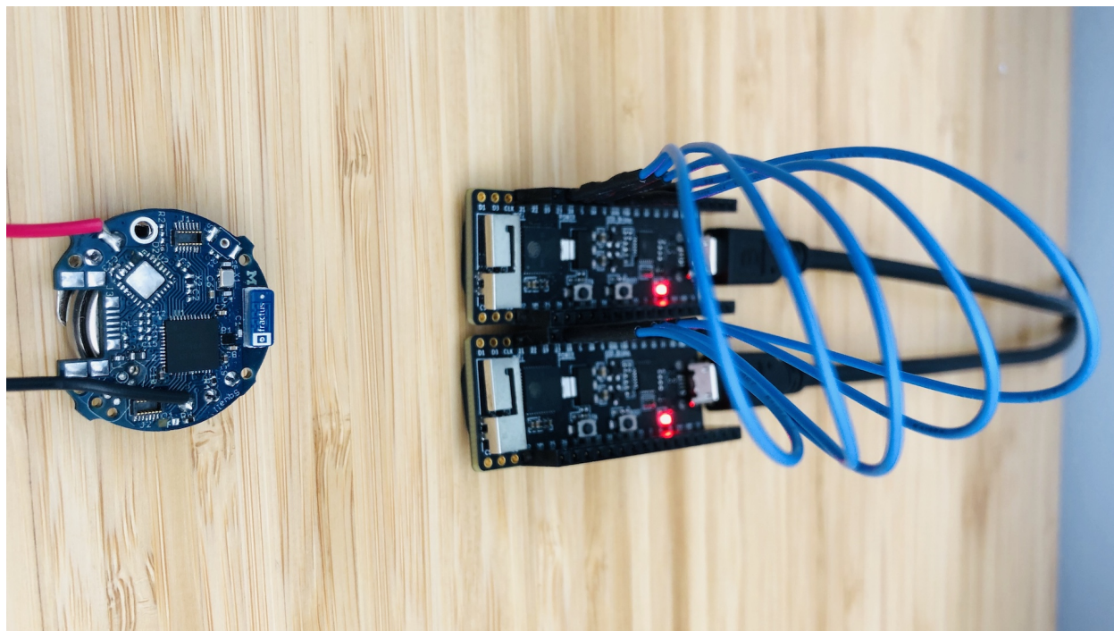
Figure 3.7: Dual-ESP gateway setup. Two ESP32 boards are connected via SPI. One ESP32 is dedicated to performing BLE scans, while the other solely sends the scanned data over Wi-Fi. This effectively yields near-optimal forwarding performance, roughly equivalent to the BLE scanner’s PRR.
