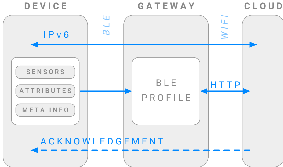
Figure 3.1: Architecture. We apply a data transport approach that considers two primary transmission mechanisms: (1) via IPv6, using the gateway as an IPv6 router and treating the peripheral as an IP-connected end host, and (2) via proxy, using the gateway to forward the device’s BLE profile to the cloud.
