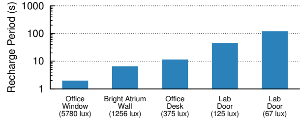
Figure 6: Recharge rate in varying lighting conditions. We measure the time the solar cell based energy-harvester takes to recharge in opportunistic trigger mode under different lighting conditions. As expected, the brighter the room the faster the recharge rate. Rooms with natural light (atrium and office) can support relatively fast recharge rates (in the 10s of seconds). Rooms with only artificial light (lab) cause the sensor to recharge more slowly, but can still support a sample every two minutes.
