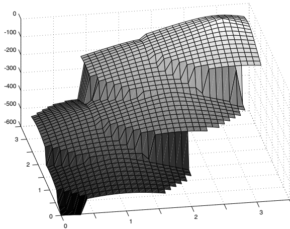
V_O^* - SMDP Value Function
