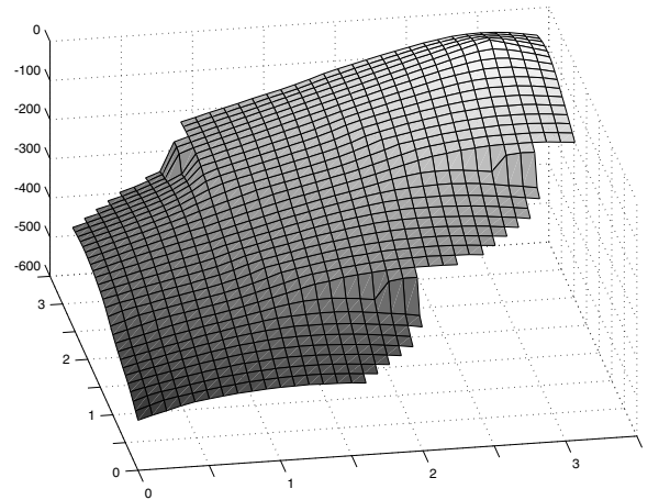
V^{\mu'} - Values with Interruption
