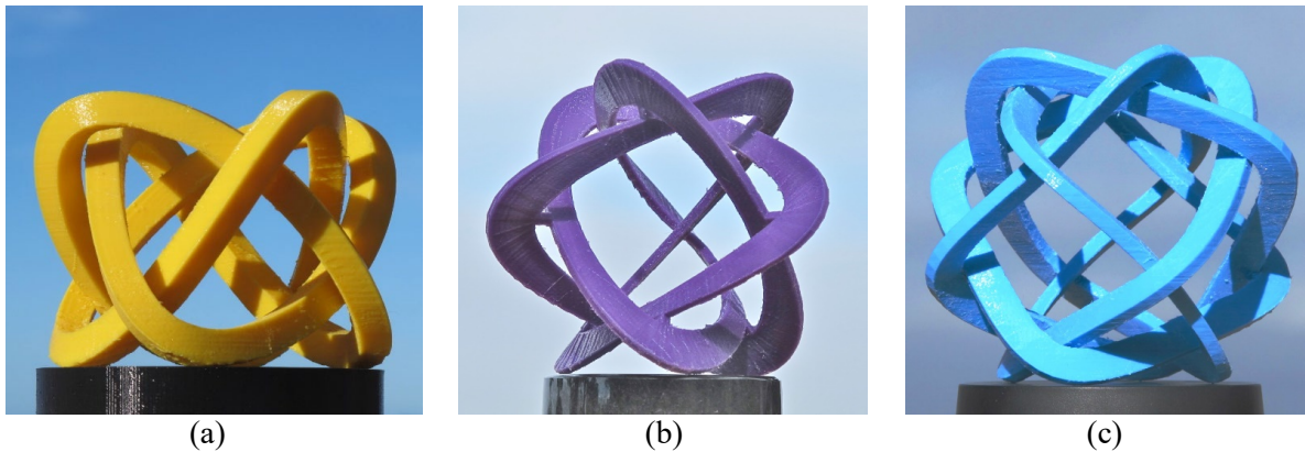
Figure 6: BallKnots ( s,t ) based on Turk's Head Knots, THK(s,t) , and their symmetries: (a) THK(4,3): S_8 ; (b) THK(3,4): D_3 ; (c) THK(4,5): S_8 .
