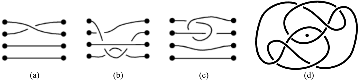
Figure 11: (a, b) Two proper representations of the same braid. (c) Not a true braid. (d) a symmetrical knot that is not a proper vortex knot.
