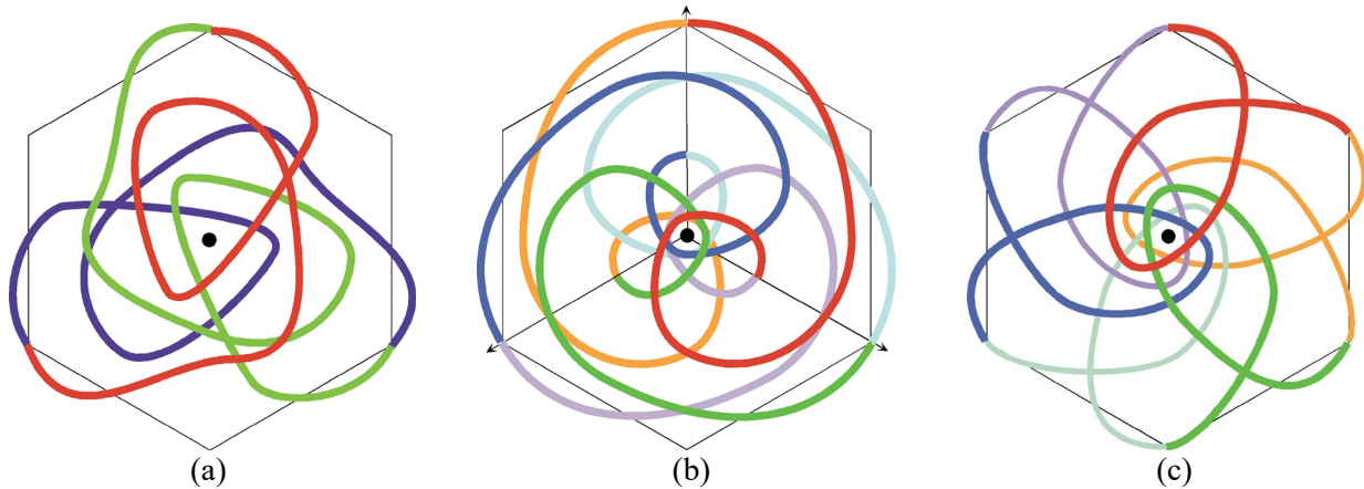
Figure 13: Knot constructions with n -fold rotational symmetry ( n=3 ): (a) C_n symmetry; (b) D_n symmetry; (c) S_{2n} symmetry.
