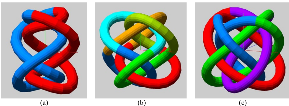
Figure 8: BallKnots , BK(s,t) , using crossover-pattern (oouu\ oouu)^s and their symmetries: (a) BK(2,5): S_4 , (b) BK(3,5): S_6 , (c) BK(4,5): S_8 .
