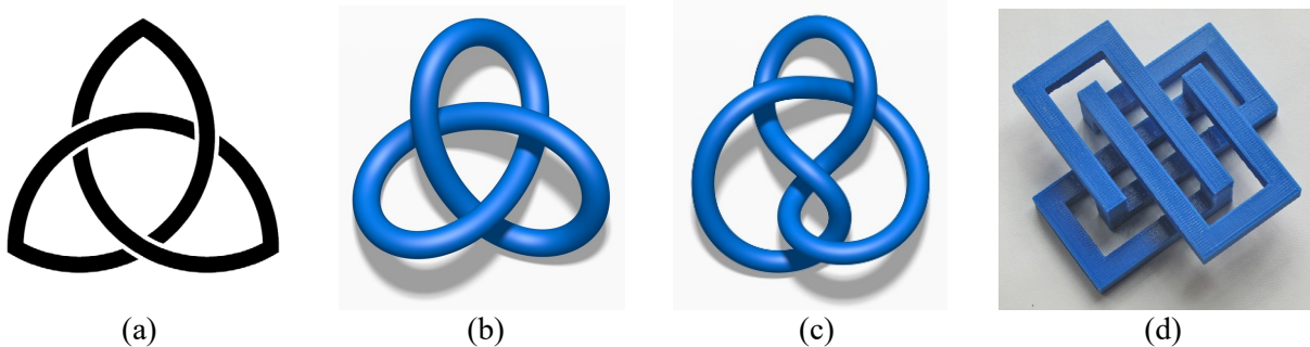
Figure 1: Trefoil-knot (Knot 3_1 ): (a) 2D diagram with C_3 symmetry; (b) 3D model with D_3 symmetry. Figure-8 knot (Knot 4_1 ): (c) 3D model with C_2 symmetry; (d) 3D model with S_4 symmetry.
