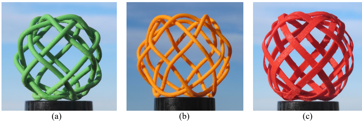
Figure 7: BallKnots ( s,t ) based on Turk's Head Knots, THK(s,t) , and their symmetries: (a) THK(5,6): D_5 ; (b) THK(6,5): S_{12} ; (c) THK(6,7): S_{12} .
