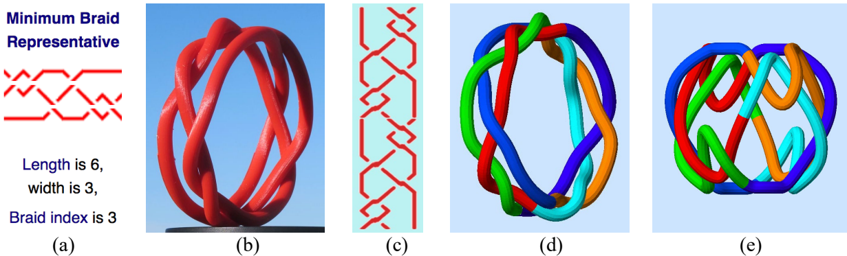
Figure 9: (a) The braid representation of Knot 6_3 , (b) Knot 6_3 as a cylindrical braid sculpture. (c) Two concatenated braids, (d) closed into a cylindrical braid, (e) formed into a ball-knot.
