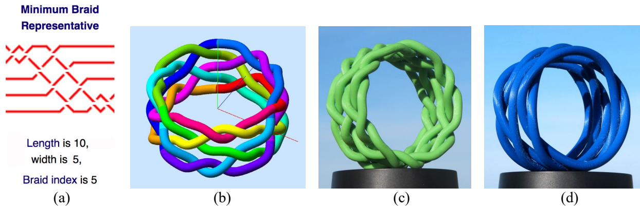
Figure 10: (a) The braid representation of Knot 10_{43} . (b) Three concatenated braids in a loop; (c) resulting sculpture with C_3 symmetry, (d) C_2 sculpture formed with 2 braid segments.
