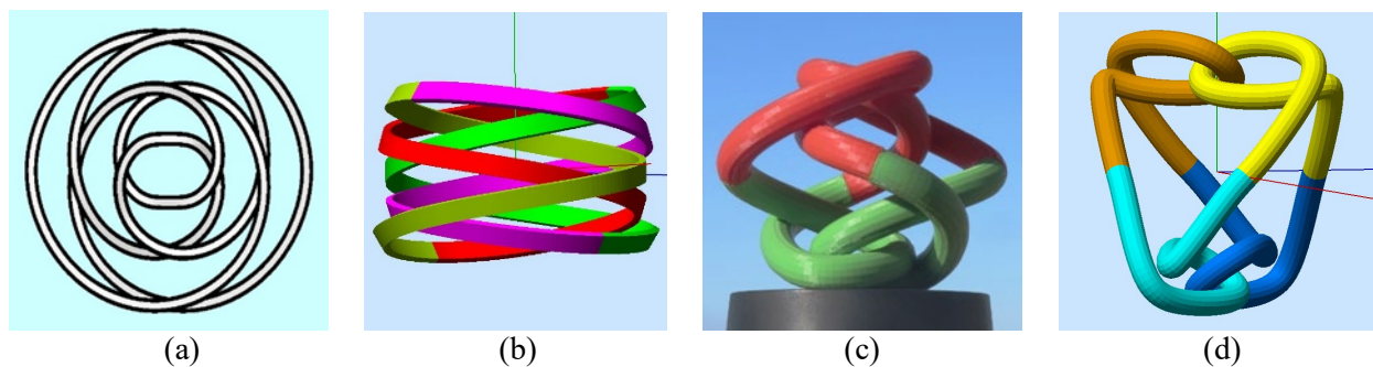
Figure 5: Knot 6_3 shown: (a) as a flat 5-strand circular braid, (b) as a cylindrical braid, (c) as a ball-knot, (d) in a tetrahedral configuration with linked top- and bottom-edges.
