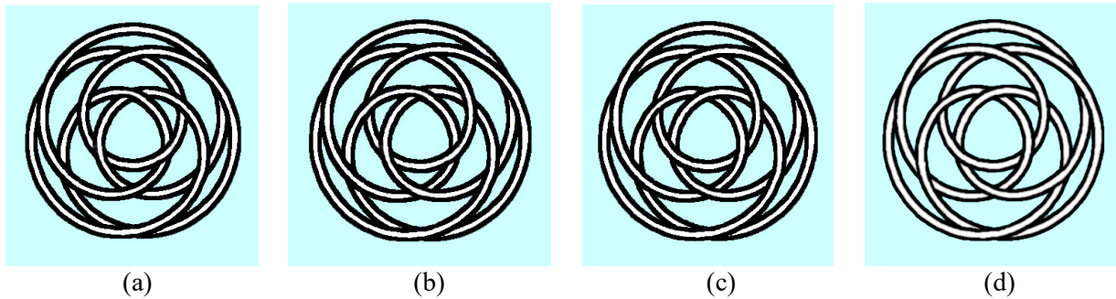
Figure 3: Circular braids: (a) (oouu\ oouu)^3 ; (b) (oouu\ oouu)^3 ; (c) (oouo\ uouu)^3 ; (d) (oouo\ uouu)^3 .
