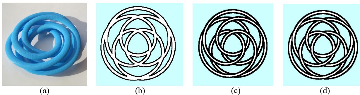
Figure 2: (a) \text{TorusKnot}(3,5) ; (b) flattened template; (c) braid representing the original knot; (d) an alternating over- under-crossing pattern, resulting in a Turk’s Head Knot.
