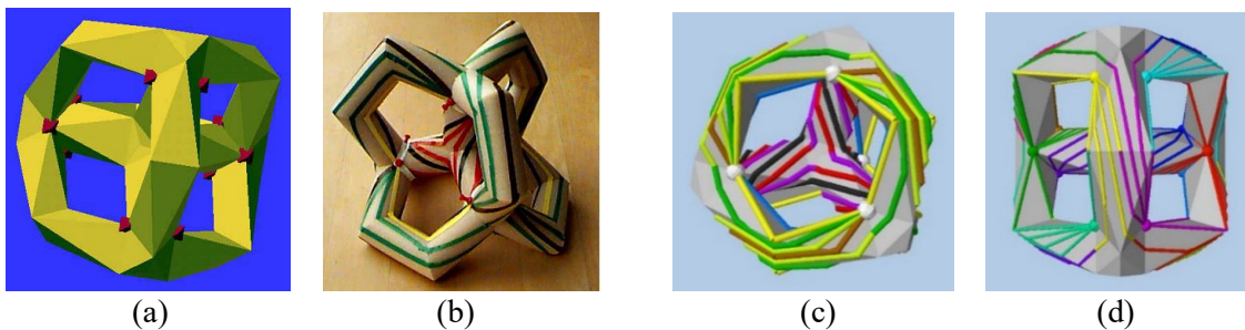
Figure 11: (a) Genus-6 handle-body with good node locations. (b) Symmetrical embedding of K_{12} . (c) 66 edges of K_{12} on polyhedral model. (d) Split edges, colored to show extent of 12 countries.
