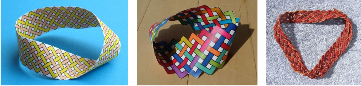
Figure 13: Möbius-twisted Turk's Head knots: (a) 2-loops, p=6 , b=31 ; (b) single thong, p=6 , b=16 ; (c) triply-twisted Möbius braid made from latigo leather, p=6 , b=34 .
