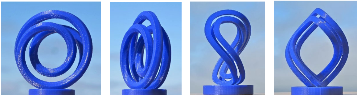
Figure 4: Un-knots: (a,b) A simple torus knot, front and side; (c,d) warped version of the same knot.
