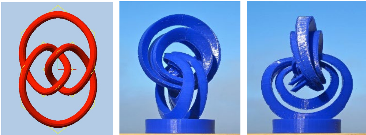
Figure 8: (a) 2-lobe layout of the Figure-8 knot. (b,c) 2-lobe variant of the Figure-8 cable-knot.
