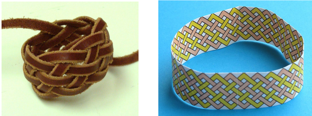
Figure. 12: (a) Single-strand latigo leather knot; p=6, b=7 . (b) Turk's Head link with 2-loops; p=6, b=32 .
