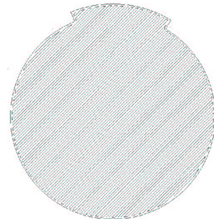
Figure 18. A SAMPLE SLICE THROUGH THE SCREW PART, USING THE QUICKSLICE SOFTWARE'S FAST BUILD OPTION. ALL OF THE ROADS ARE DENSELY SPACED.
