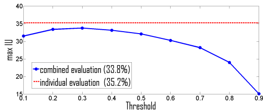
Figure 4. Calibration of multiple detectors through pixel classification.
