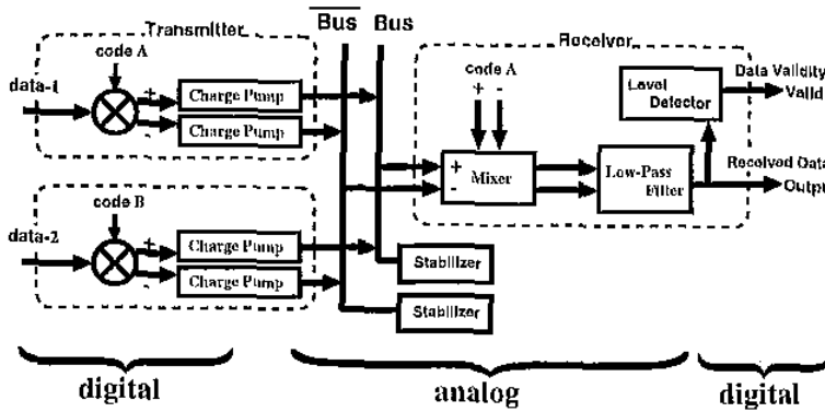
Figure 22.5.1: Interface block diagram.
