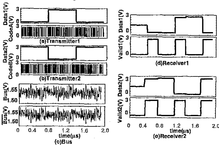
Figure 22.5.5: Simulation results of entire circuit for two-to-two communication. Figures show input data and PN code in transmitters (a) 1 and (b) 2, (c) signals on differential bus, and output data and valid signals in receivers (d) 1 and (e) 2.
