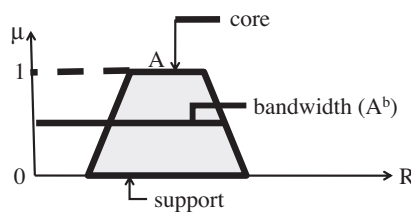
Fig. 3. Interval-valued approximation to a trapezoidal fuzzy set.
