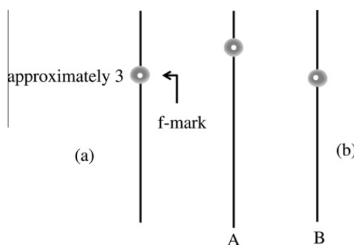
Fig. 2. (a) f -mark of approximately 3; (b) f -marks of a Z -number.
