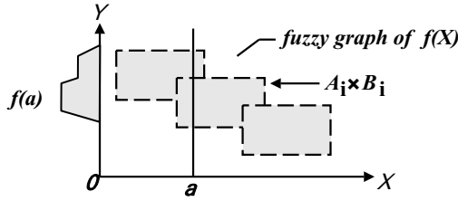
Fig. 27. Mamdani interpolation.
