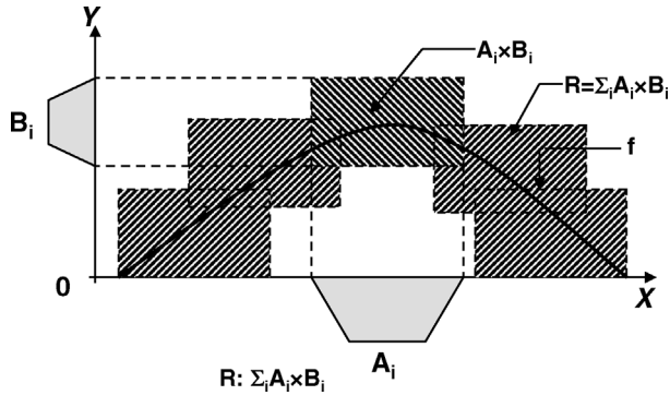
Fig. 4. Fuzzy graph.
