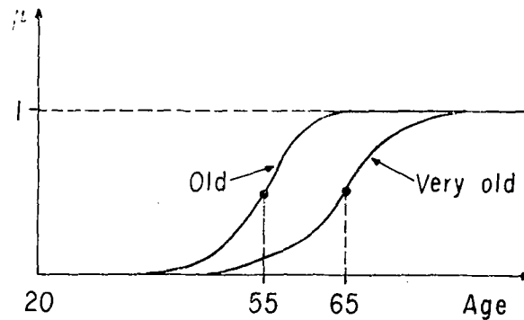
FIGURE 2. Representation of “very” as a function from \mathcal{F}(K) to \mathcal{F}(K) .
