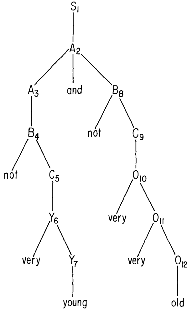
FIGURE 3. Syntax tree for x = \text{not very young and not very very old} .
