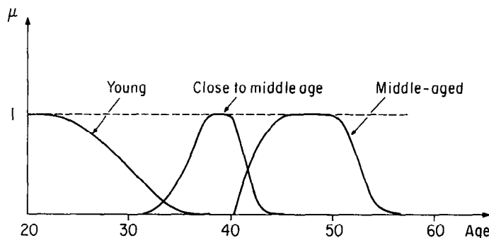
FIGURE 1. Characterization of “young,” “close to middle-age” and “middle-aged” as fuzzy sets in U .
