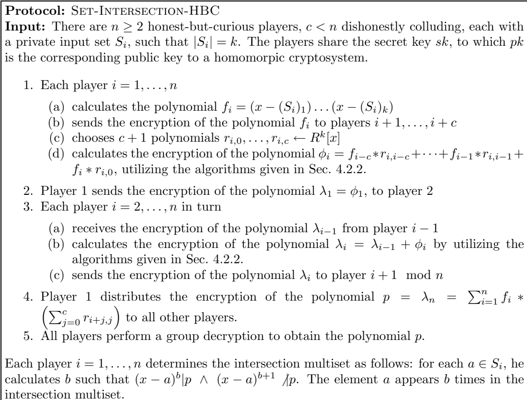
Figure 1: Set-Intersection protocol for the honest-but-curious case.
