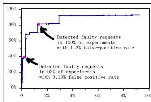
Figure 1: Detection rate vs. false positive rate for PCFG-based path-shape analysis of PetStore 1.3 running on our modified JBoss server. Relying on HTTP error logs would reduce the detection rate to about 78%. Compared to the uninstrumented application, our throughput is 17% less, request latency is about 40ms more, and analysis of several thousand paths takes a few seconds, suggesting that the approach is feasible as an online technique.
